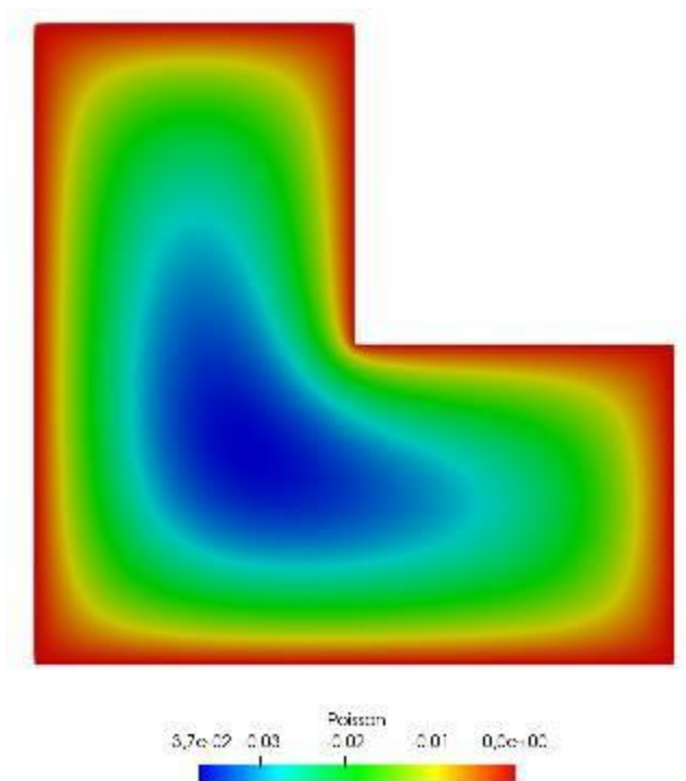
Fig. 4. Temperature level for the heat equation; Poisson's equation, with boundary conditions on input heat, [6]. Remark. In FEM, the Lagrangian element has an exact Gaussian integration, and other formats are e.g. serendipity elements
