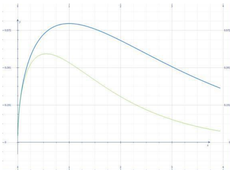
Fig. 7. Pressure function (4), p(y)/-P=ym \exp(-s*y) with parameter m<2/3 , such that the power (6) is singular at origin. Upper curve m=0.5, s=0.5 . Lower curve m=0.5, s=0.9
